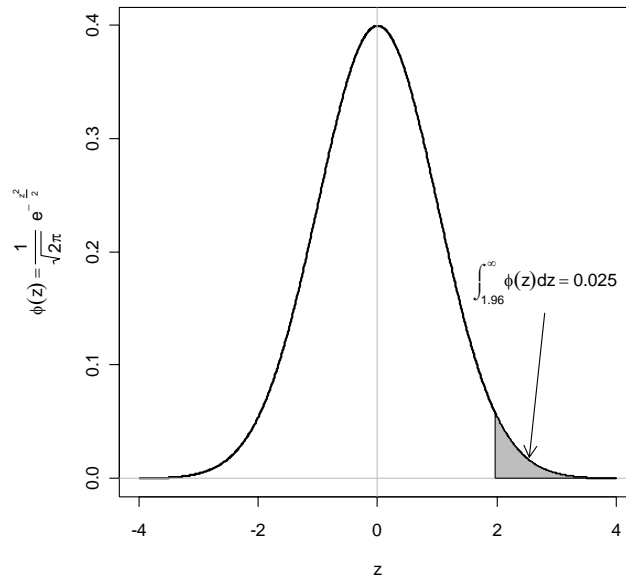
The Standard Normal Density Function \phi(z)
