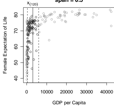
(c) Weighted Average (Kernel Estimate)
