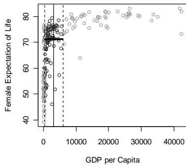
(c) Weighted Average (Kernel Estimate)
