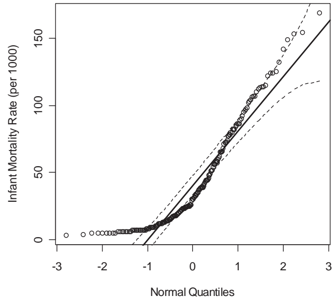
Figure 6. Normal quantile-comparison plot for infant mortality.
