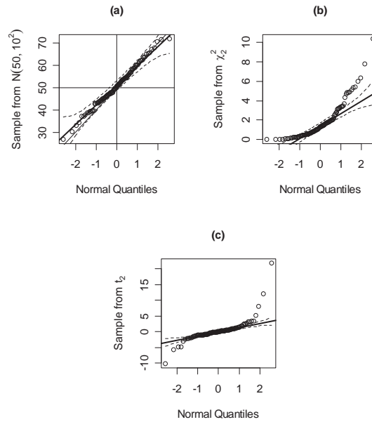
Figure 5. Normal quantile comparison plots for samples of size n = 100 drawn from three distributions.
