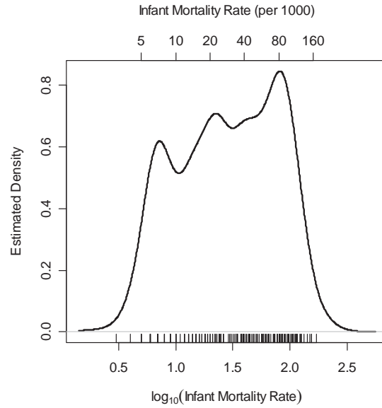
Figure 15. Adaptive-kernel density estimate for log-transformed infant mortality.
