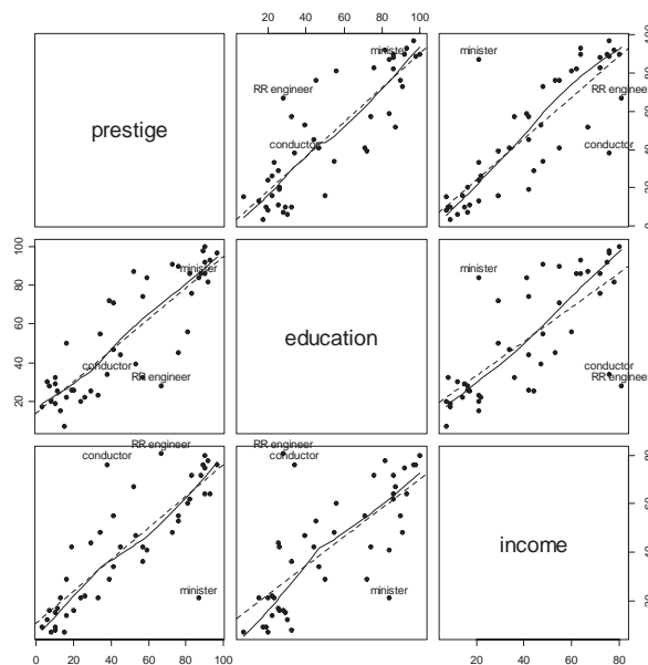
Figure 11. Scatterplot matrix for prestige, income, and education in Duncan's occupational prestige data.
