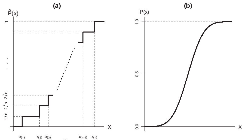
Figure 4. (a) Typical ECDF; (b) typical CDF.
