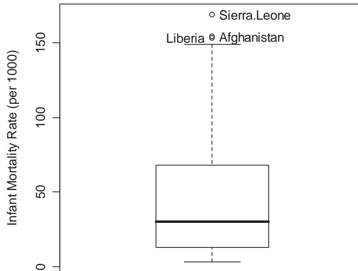
Figure 7. Boxplot of infant mortality.
