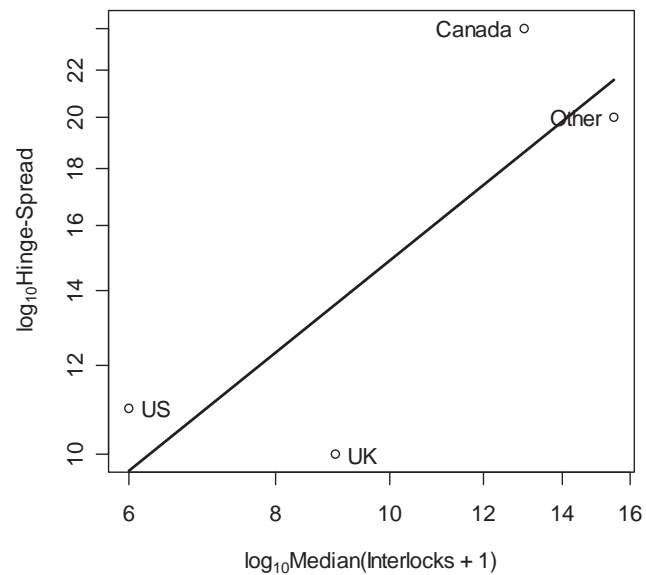
Figure 21. Spread-level plot for Ornstein's interlocking-directorate data.
