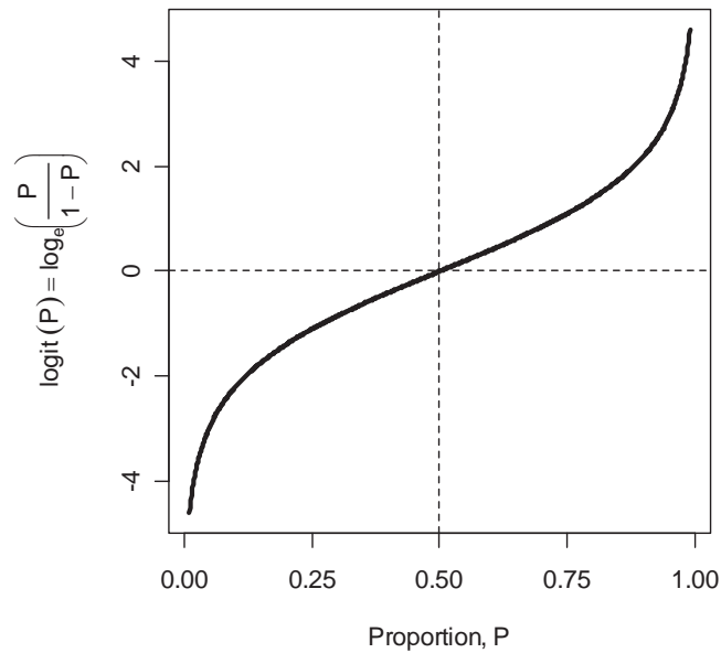
Figure 24. The logit transformation of a proportion.
