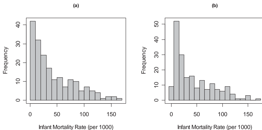
Figure 2. Two histograms with the same bin width but different origins for infant mortality in the United Nations data.
