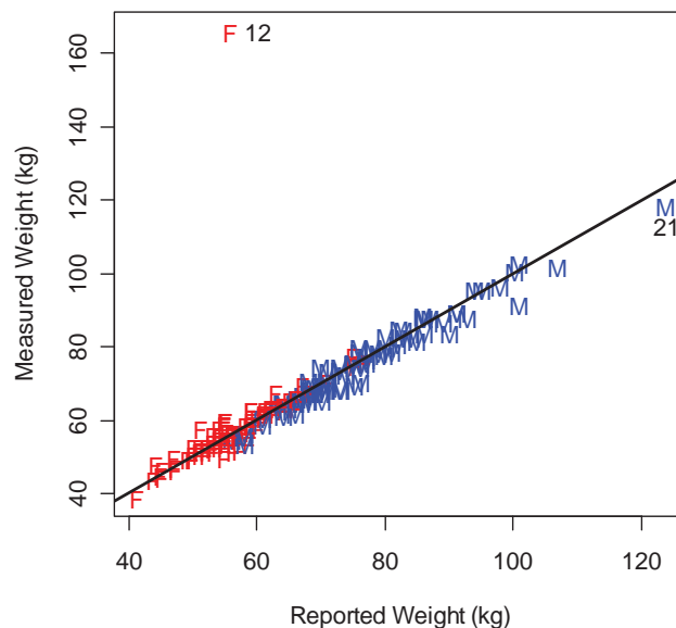
Figure 12. Measured by reported weight for 183 men (M) and women (F) engaged in regular exercise.
