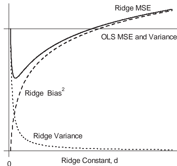
Figure 3. The squared bias, variance, and MSE of the ridge estimator as a function of the ridge constant, compared to the MSE of the OLS estimator.
